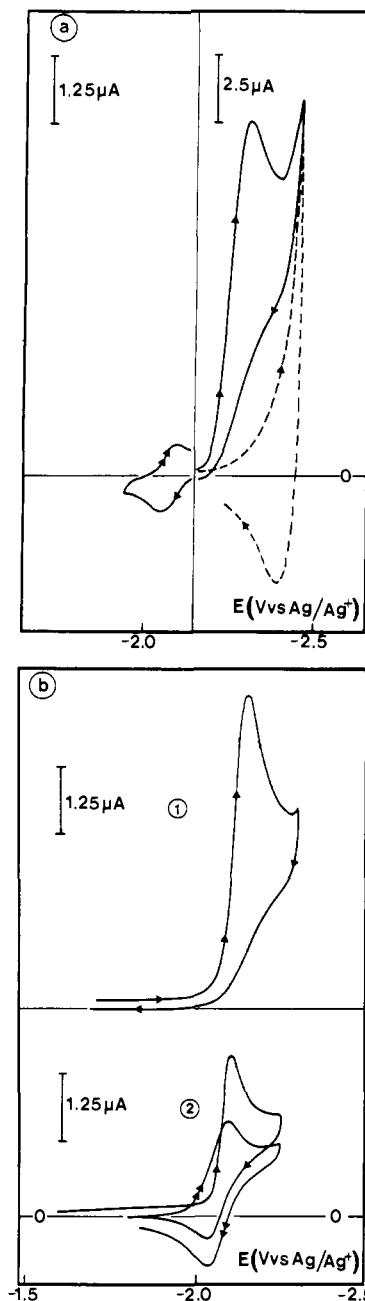
Figure 4. Cyclic voltammetry of chlorobenzene and diphenyl sulfide in liquid NH 3 + 0.1 M KBr at -38 °C, in the presence of potassium diethyl phosphite (0.11 M) at 0.2 V s -1 . (a) PhCl (4.6 mM). The dotted line shows the response of the supporting electrolyte, the anodic trace corresponding to the injection of the solvated electrons from the electrode into the solution. (b) PhSPh (2 mM) in the absence (1) and presence (2) of diethyl phosphite ions.
