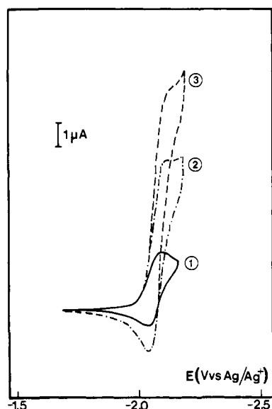
Figure 5. Cyclic voltammetry of diethyl phenyl phosphite (2 mM) in liquid \text{NH}_3 + 0.1 M KBr at -38^\circ\text{C} in the presence of 0.275 M (\text{EtO})_2\text{POK} in the absence (—) and presence of 9.3 mM (---) and 17.5 mM (- - -) PhCl: Sweep rate, 0.2 \text{ V s}^{-1} .
