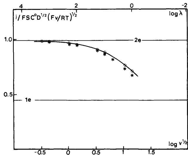
Figure 1. Cyclic voltammery of PhSPH in liquid \text{NH}_3 + 0.1 \text{ M KBr} at -38^\circ\text{C} . Variations of the cathodic peak current ( i_p ) with this sweep rate ( v in \text{V s}^{-1} ): (O) without addition of \text{PhS}^- , PhSPH conc ( C^0 ) = 3 mM. (*) in the presence of 0.11 M \text{PhS}^- , PhSPH conc ( C^0 ) = 2.8 mM. The solid line is the DISP1 working curve represented as a function of the dimensionless kinetic parameter \lambda = RTk_1/Fv (upper horizontal scale). Lower horizontal scale: v in \text{V s}^{-1} . i = current intensity, S = electrode surface area, C^0 = concn. of PhSPH, D = diffusion coefficient. i/FS C^0 D^{1/2} (Fv/RT)^{1/2} is a dimensionless quantity.
